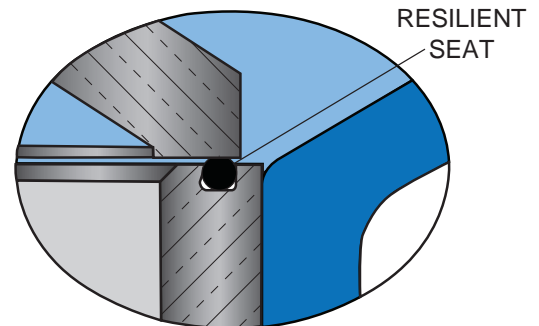
Figure 3 - Resilient Seating Detail at Low Pressure
